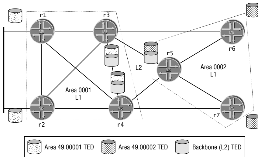
FIGURE 2.6 Varying TED views
