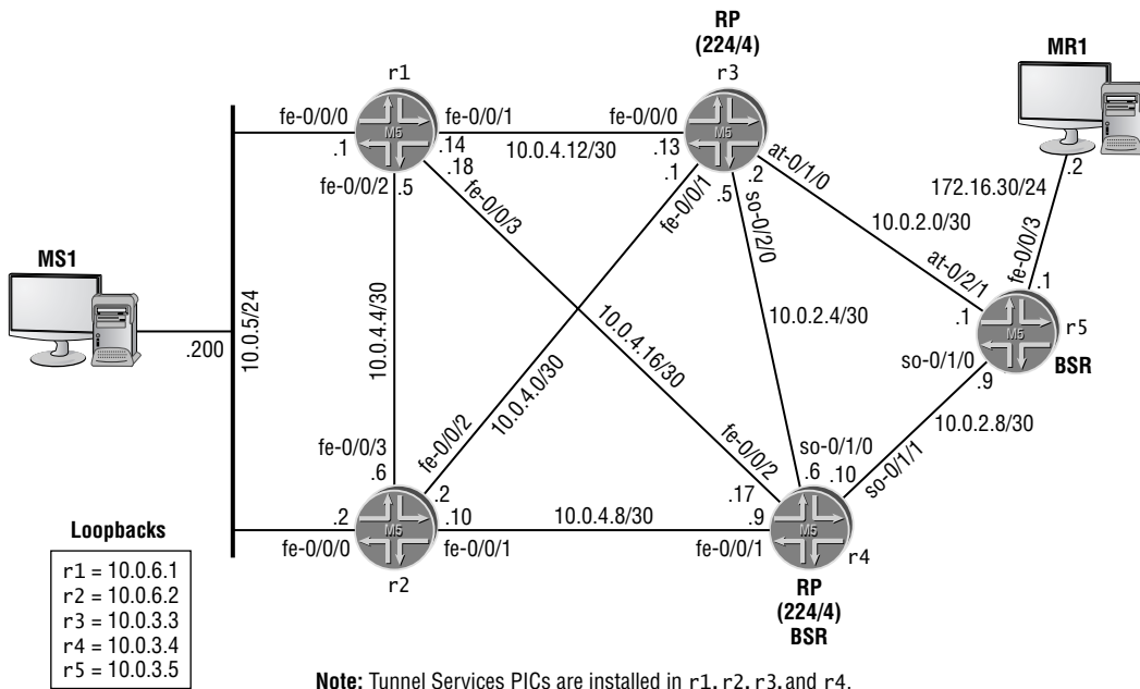
FIGURE 4.5 PIM-SM topology
