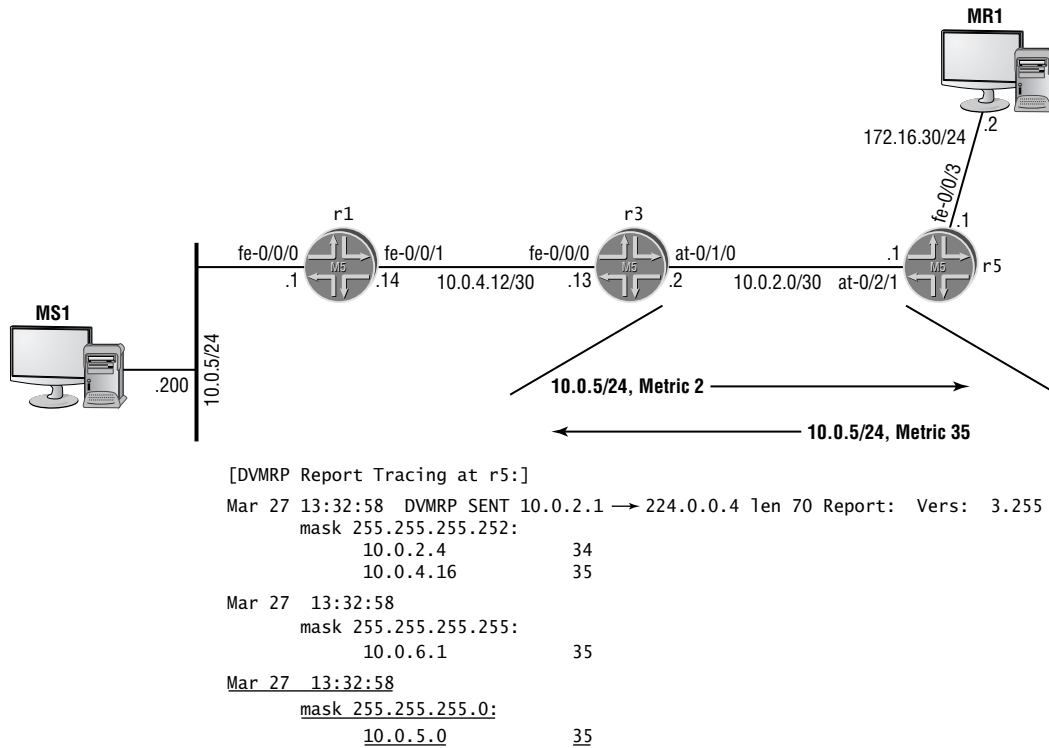
FIGURE 4.3 DVMRP poison reverse
