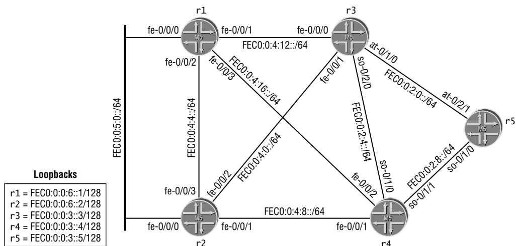
FIGURE 5.2 IPv6 topology and addressing
