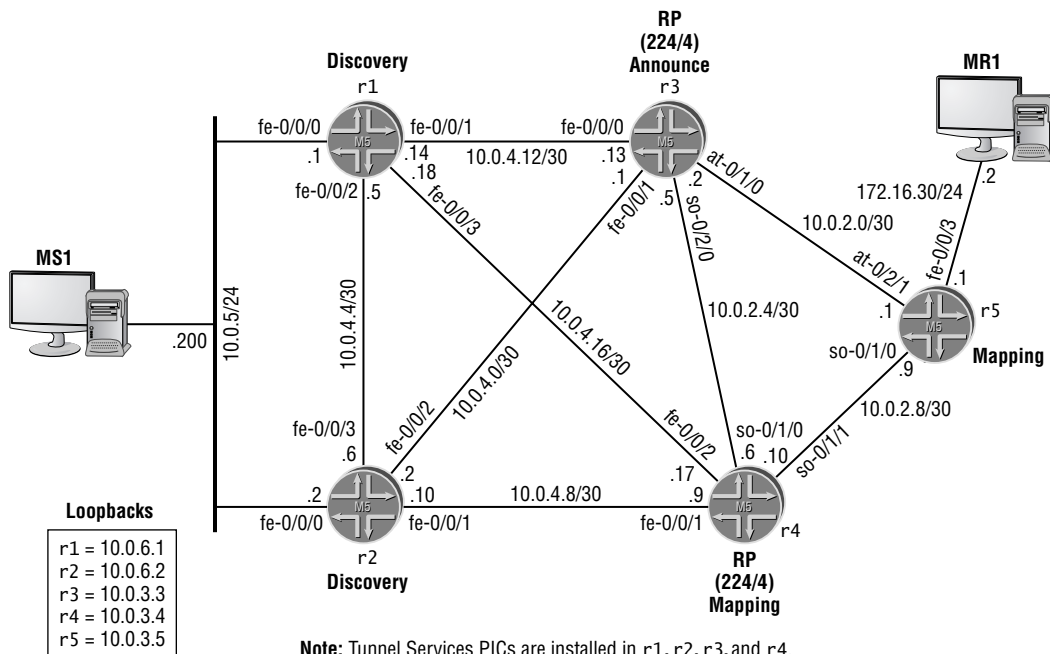
FIGURE 4.6 Auto-RP topology
