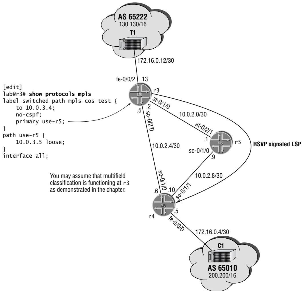
FIGURE 6.3 CoS topology
