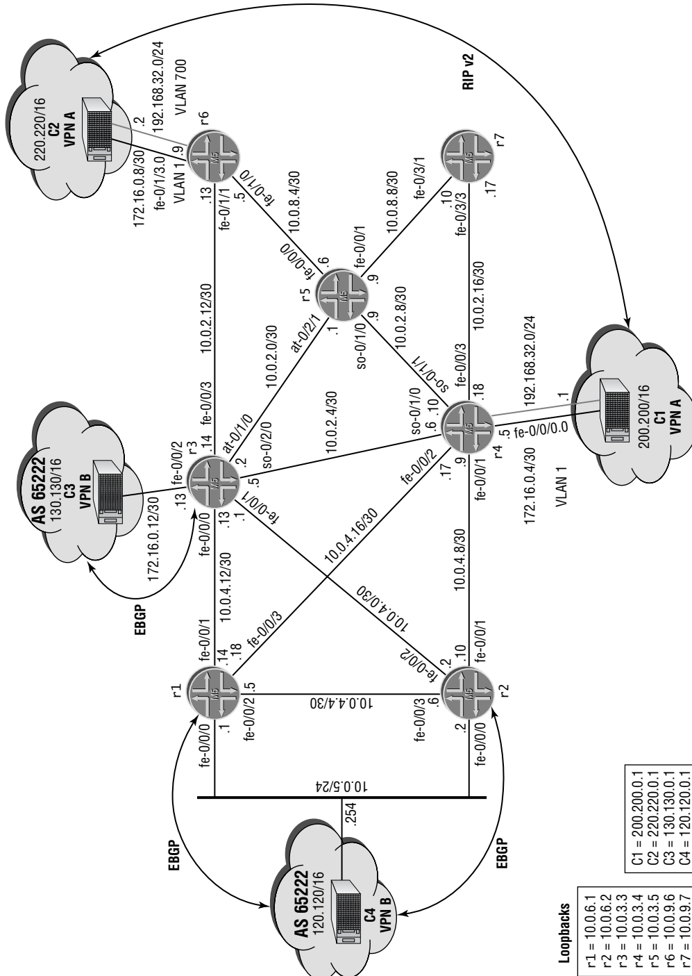
FIGURE 7.8 MPLS case study topology
