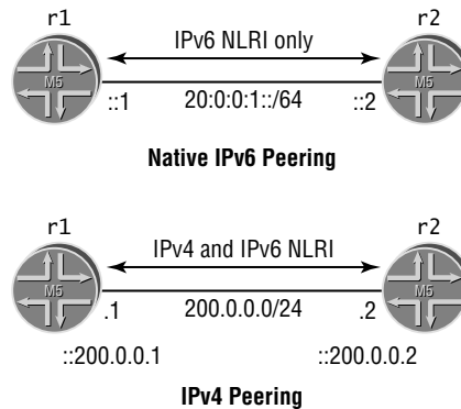
FIGURE 5.6 IPv6 BGP support options
