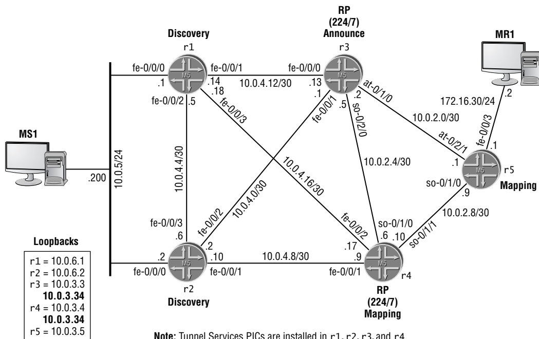
FIGURE 4.7 Any-Cast topology
